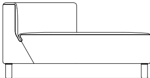
Couch 140 (Left,Right) w140 d70 h68 sh43.5
